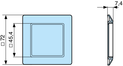
Adaptor for 72 x 72 mm cut-out: 26546842
