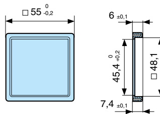
Adaptor for 55 x 55 mm cut-out: 26546846
